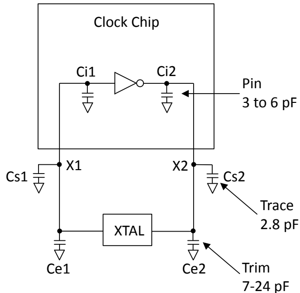
Figure 5.2. Crystal Loading Example
