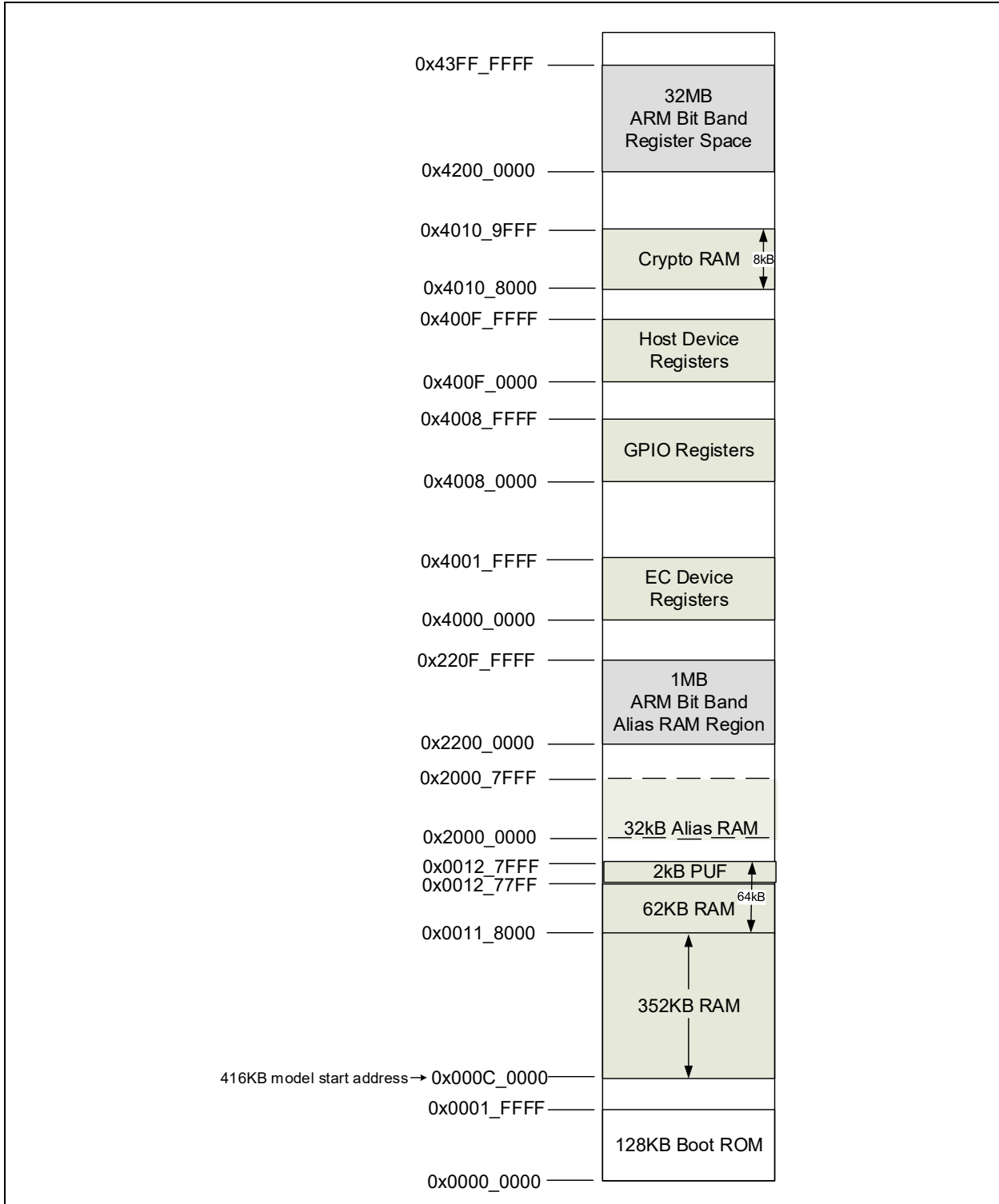
FIGURE 6-1: MEMORY LAYOUT
