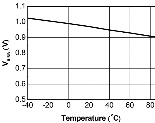
Figure 28. V_{IUSB} vs T_A V_{USB}=5.0 V, R_{IUSB}=9.76 k \Omega , V_{BAT}=3.7 V
