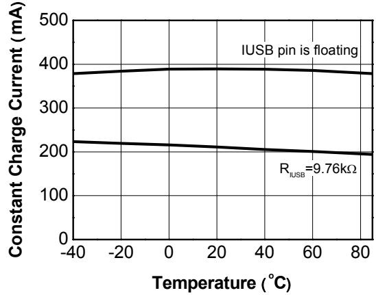
Figure 30. USB Charger CC Current vs T_A V_{USB}=5.0 V, V_{BAT}=3.7 V
