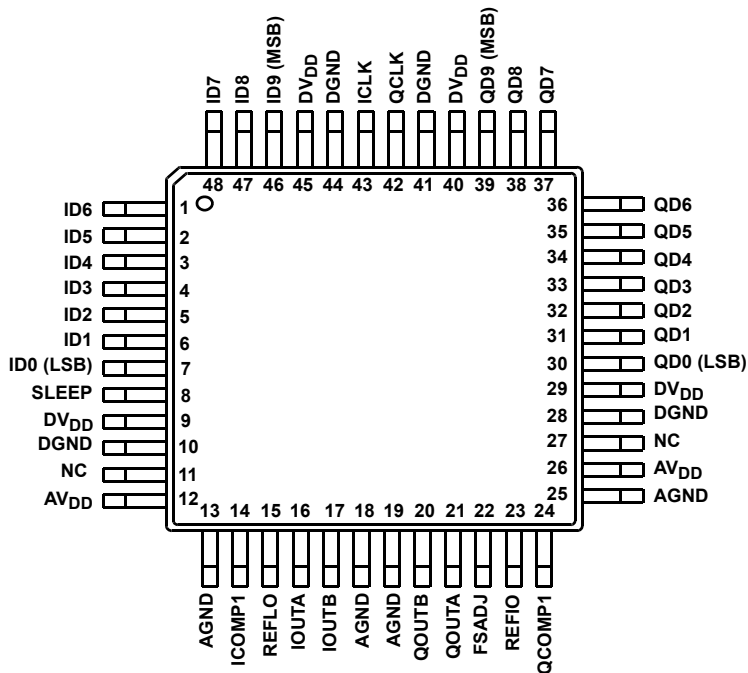
HI5728 (48 LD LQFP) TOP VIEW
