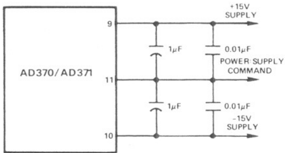
Figure 2. Power Supply Decoupling
