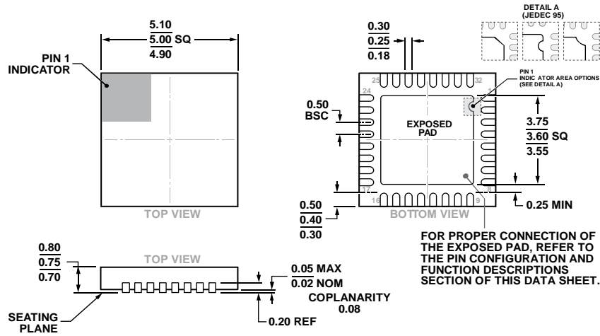
Figure 61. 32-Lead Lead Frame Chip Scale Package [LFCSP] 5 mm x 5 mm Body and 0.75 mm Package Height (CP-32-12) Dimensions shown in millimeters
