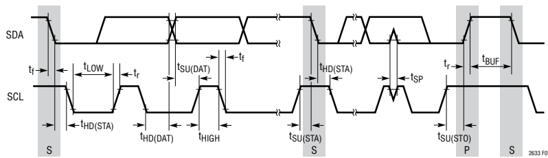
Figure 1. I 2 C Timing
