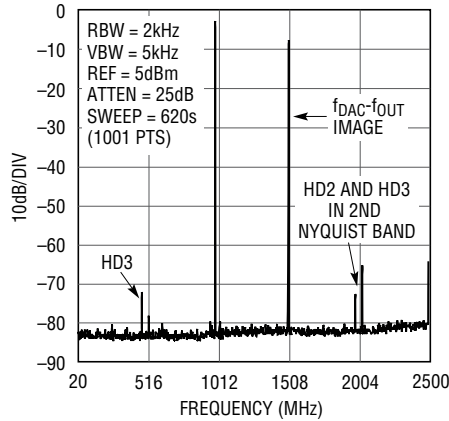
Single-Tone Spectrum at f_{OUT} = 990MHz , f_{DAC} = 2.5Gsp/s
