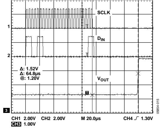
Figure 14. Full-Scale Settling Time, 5 V
