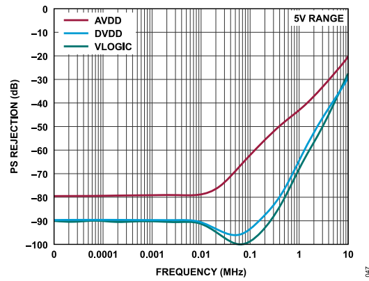
Figure 59. AC PSRR
