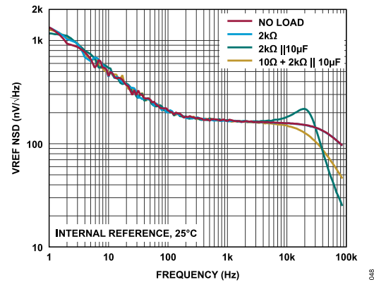
Figure 60. Reference Voltage ( V_{REF} ) NSD vs. Frequency, Load Impedance
