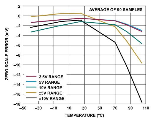
Figure 30. Zero-Scale Error vs. Temperature
