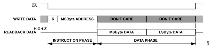
Figure 70. Multibyte Register Read with Descending Addressing
