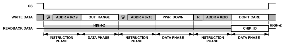
Figure 71. Single Instruction Mode Register Access Example with Address Descending
