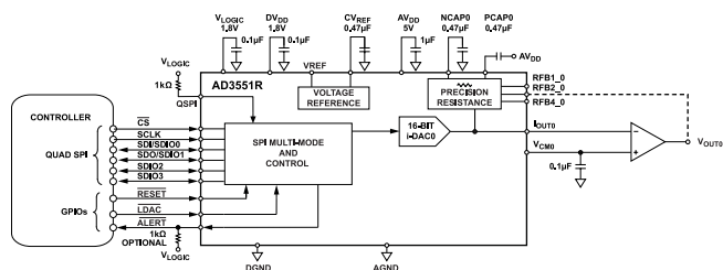
Figure 90. AD3551R Application Diagram with Quad SPI
