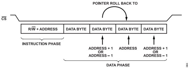
Figure 74. Looping Enabled with STREAM_MODE = 2
