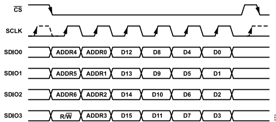
Figure 83. Quad SPI Mode
