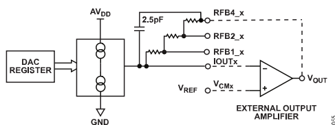
Figure 66. DAC Channel Architecture Block Diagram
