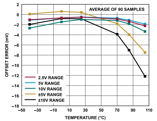
Figure 29. Offset Error vs. Temperature
