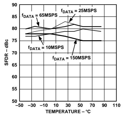
Figure 21. "In-Band" Single-Tone SFDR vs. Temperature @ f_{OUT} = f_{DATA}/11 , A_{OUT} = 0 dBFS
