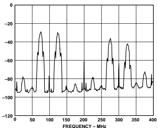
Figure 51. Spectral Plot of 16-QAM Signal in Direct IF Mode at f_{DATA} = 100 MSPS
