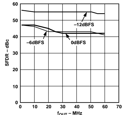
Figure 12. "Out-of-Band" SFDR vs. f_{OUT} @ f_{DATA} = 150 MSPS
