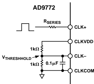
Figure 37. Single-Ended Clock Interface
