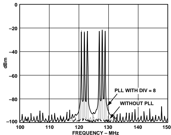
Figure 28. Direct IF Mode Reveals Phase Noise Degradation With and Without PLL Clock Multiplier (IF = 125 MHz and f_{DATA} = 100 MSPS)
