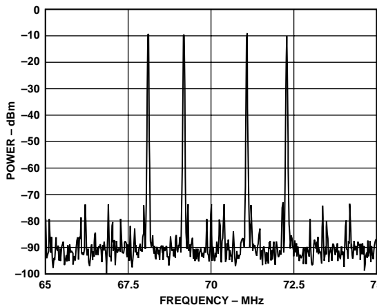
Figure 53. Spectral Plot of Four Carriers at 70 MHz IF with f_{DATA} = 52 MSPS, PLLVDD = 0
