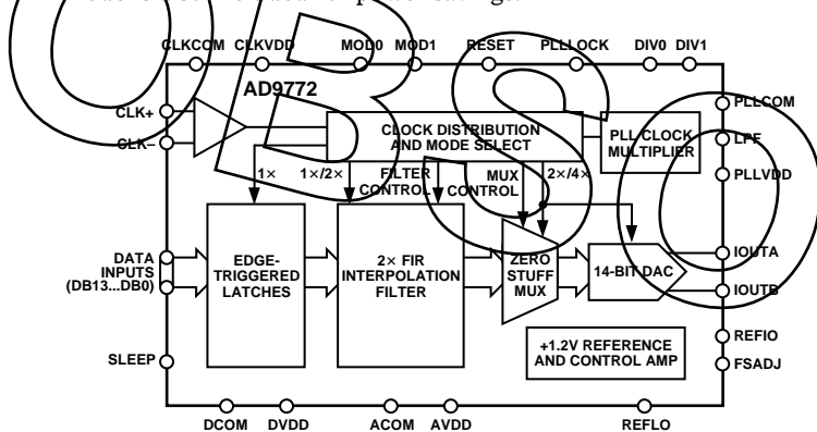
Figure 22. Functional Block Diagram
