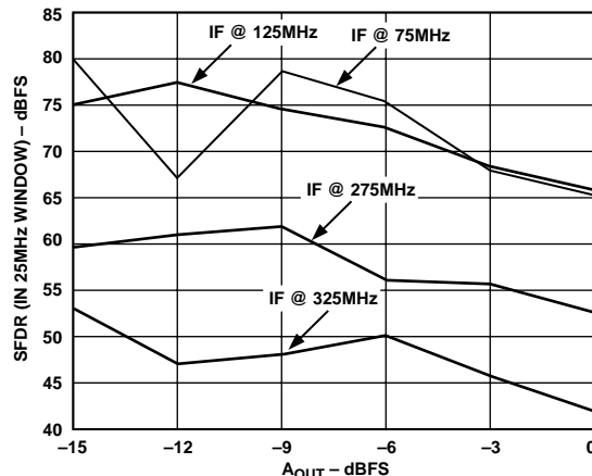
Figure 52. Dual Tone “Windowed” SFDR vs. A_{OUT} at f_{DATA} = 100 MSPS
