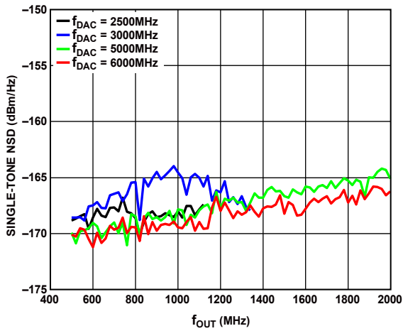
Figure 25. Single-Tone NSD Measured at 70 MHz vs. f_{OUT} over f_{DAC}
