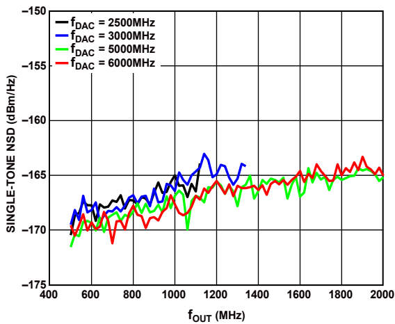
Figure 26. Single-Tone NSD Measured at 10% Offset from f_{OUT} vs. f_{OUT} over f_{DAC}
