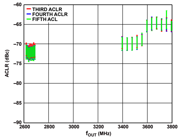
Figure 59. Four-Carrier, W-CDMA ACLR vs. f_{OUT} (Third ACLR, Fourth ACLR, Fifth ACLR)
