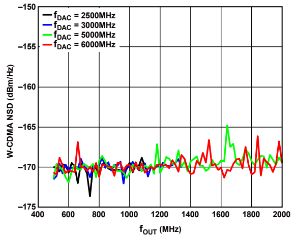
Figure 27. W-CDMA NSD Measured at 70 MHz vs. f_{OUT} over f_{DAC}
