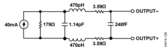
Figure 141. Equivalent Circuit Model of the DAC Output
