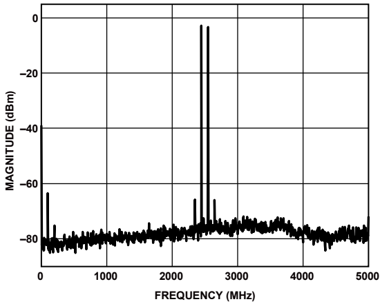
Figure 42. Single-Tone Spectrum at f_{OUT} = 2350 \text{ MHz}
