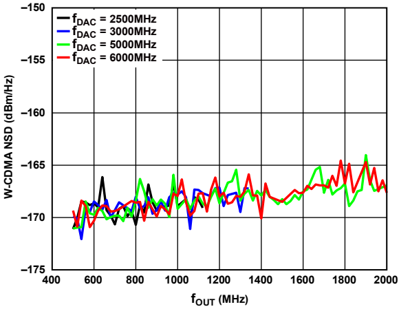
Figure 28. W-CDMA NSD Measured at 10% Offset from f_{OUT} vs. f_{OUT} over f_{DAC}
