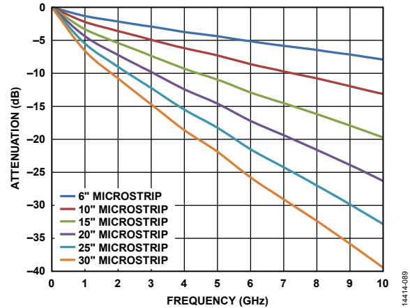
Figure 97. Insertion Loss of 50 Ohm Microstrips on FR4
