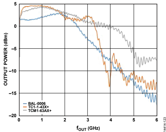
Figure 139. Measured DAC Output Response; f_{DAC} = 6 GSFS
