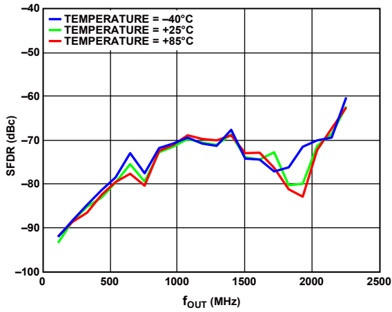
Figure 24. SFDR vs. f_{OUT} over Temperature
