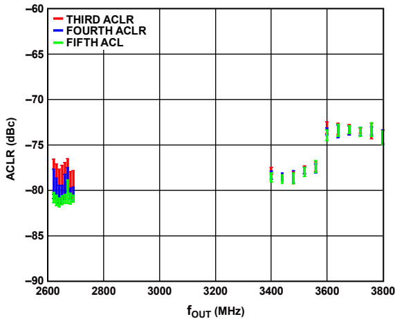
Figure 56. Single-Carrier, W-CDMA ACLR vs. f_{OUT} (Third ACLR, Fourth ACLR, Fifth ACLR)
