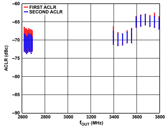
Figure 58. Four-Carrier, W-CDMA ACLR vs. f_{OUT} (First ACLR, Second ACLR)
