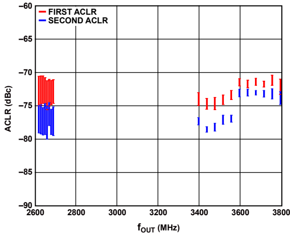
Figure 55. Single-Carrier, W-CDMA ACLR vs. f_{OUT} (First ACLR, Second ACLR)
