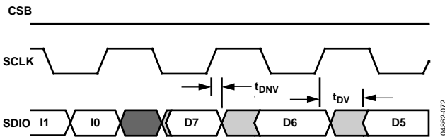
Figure 74. Timing Diagram for SPI Register Read
