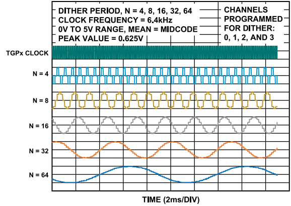
Figure 20. Sinusoidal Dither Waveform
