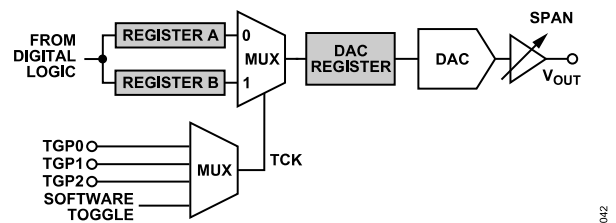
Figure 53. Toggle Operation
