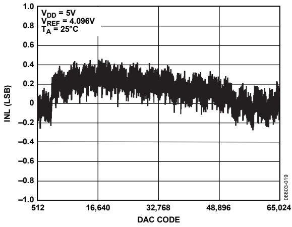
Figure 8. AD5064/AD5064-1 INL
