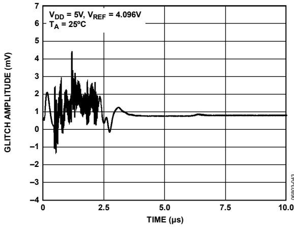
Figure 32. Analog Crosstalk
