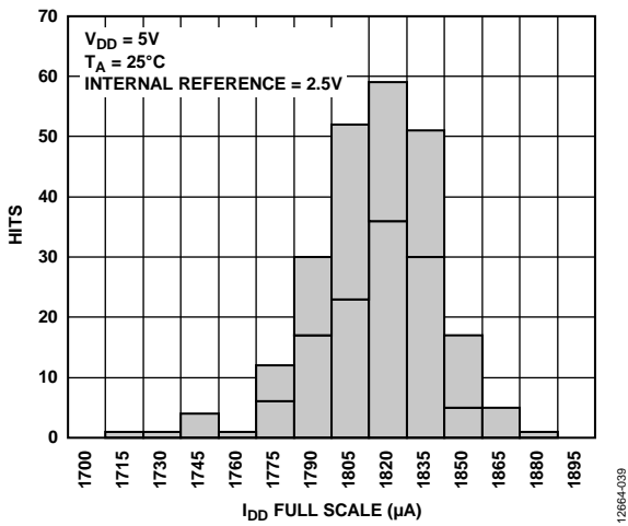
Figure 31. I_{DD} Histogram with Internal Reference
