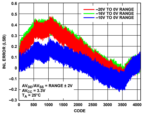
Figure 8. AD5767 INL Error vs. DAC Code (Unipolar Output)
