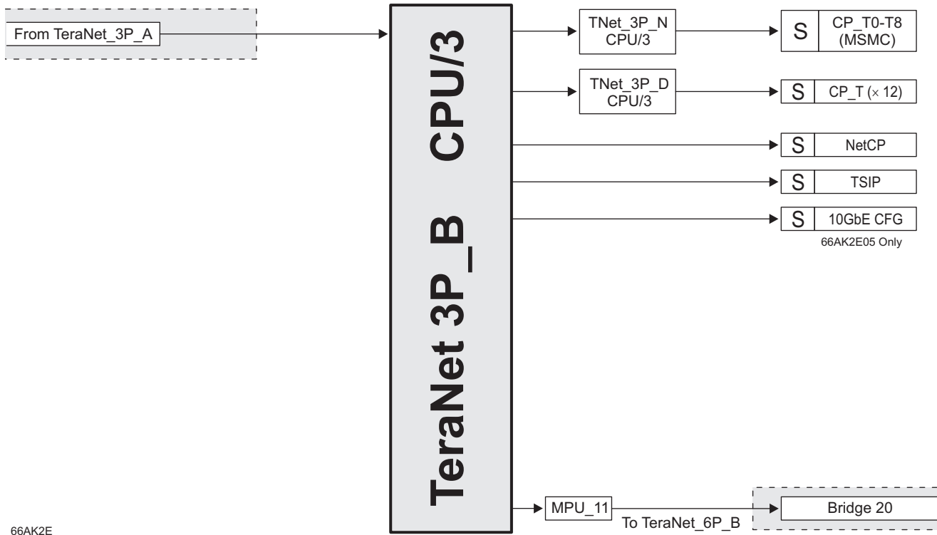
Figure 8-6. TeraNet 3P_B
