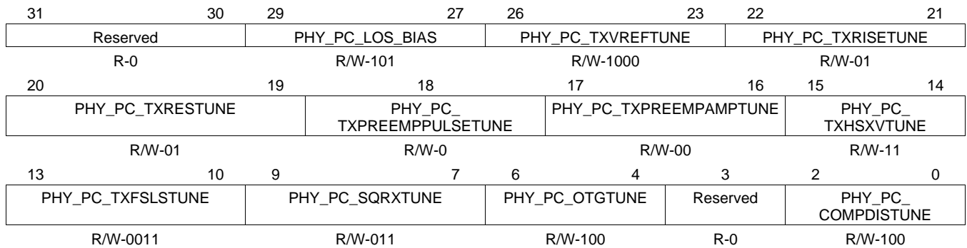
Figure 9-39. USB_PHY_CTL2 Register
