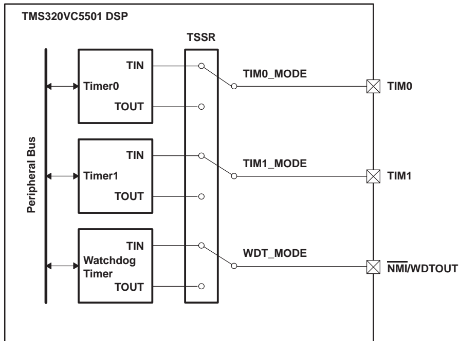
Figure 3–7. Timer Pins
