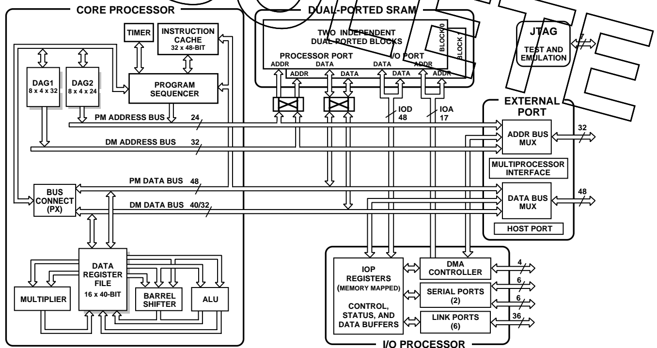
Figure 1. ADSP-21060 Processor Block Diagram (Core of the AD14160/AD14160L)
