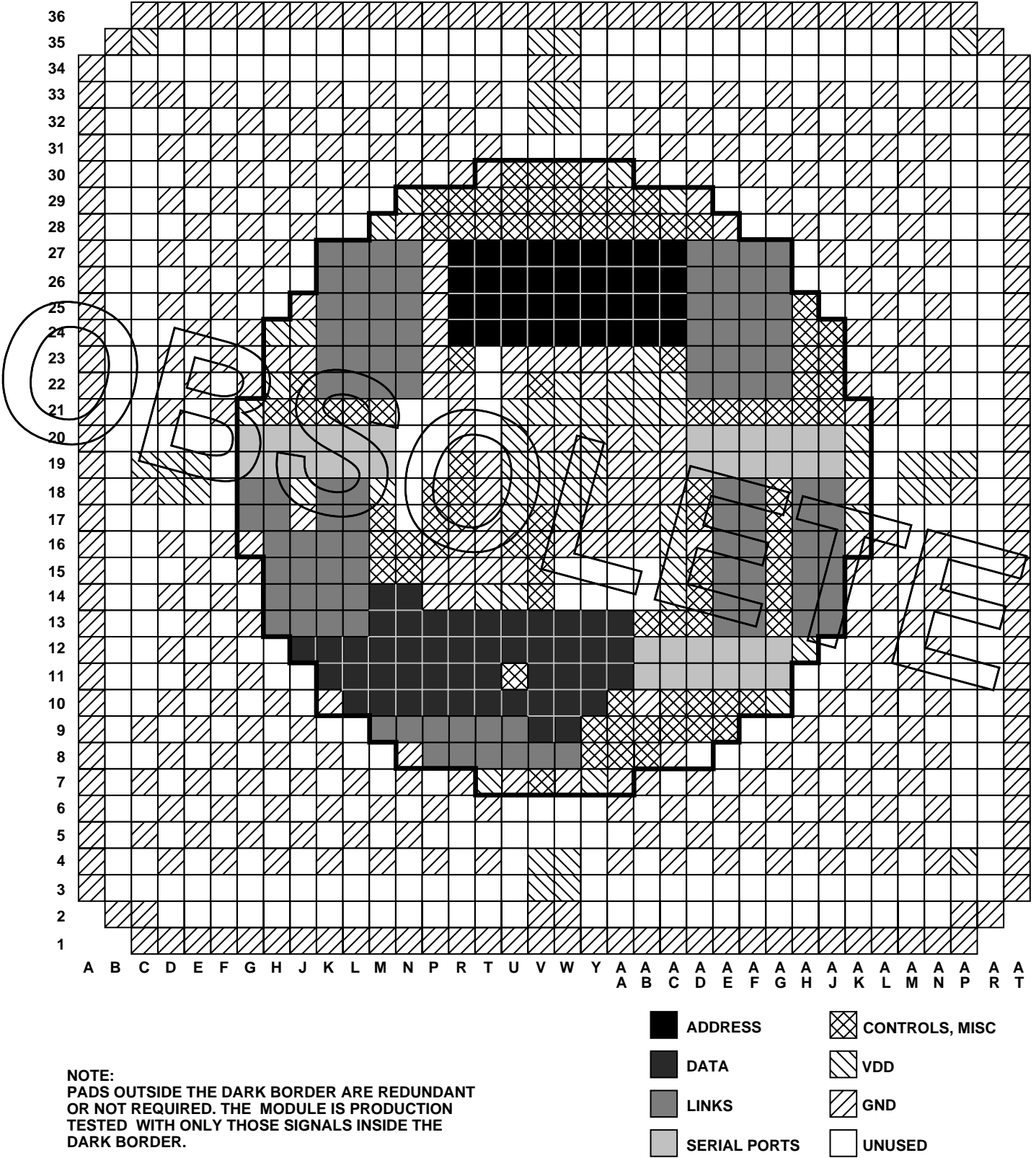
Figure 42. Board Footprint for AD14160/AD14160L Quad SHARC BGA
