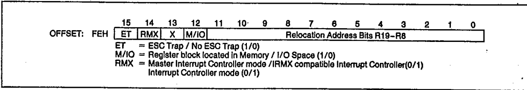
Figure 9. Relocation Register
