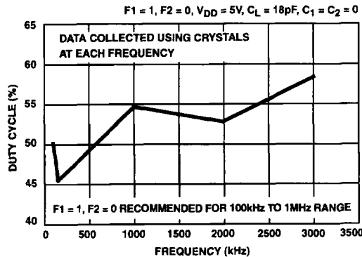
FIGURE 27. DUTY CYCLE vs FREQUENCY
