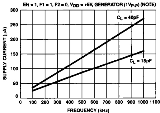
FIGURE 21. SUPPLY CURRENT vs FREQUENCY
