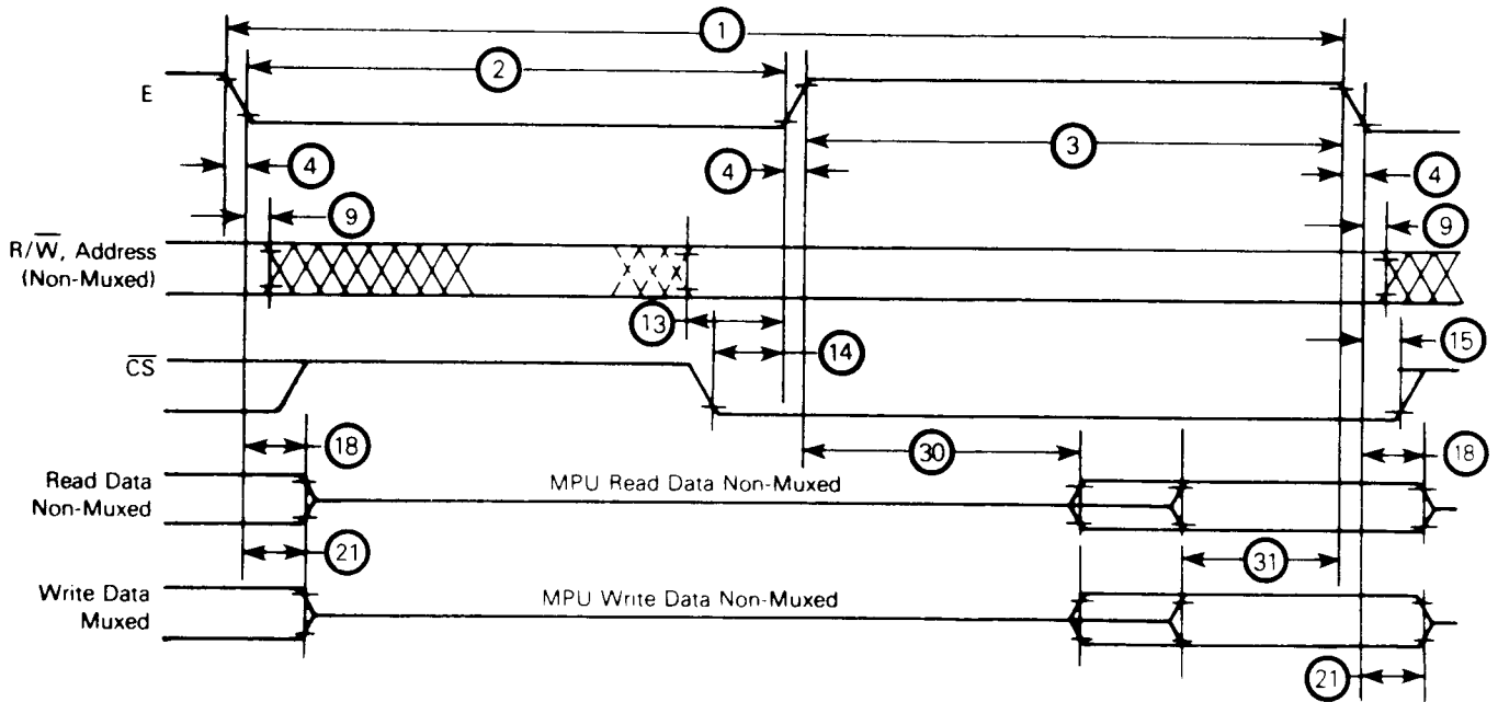
FIGURE 1 — BUS TIMING
